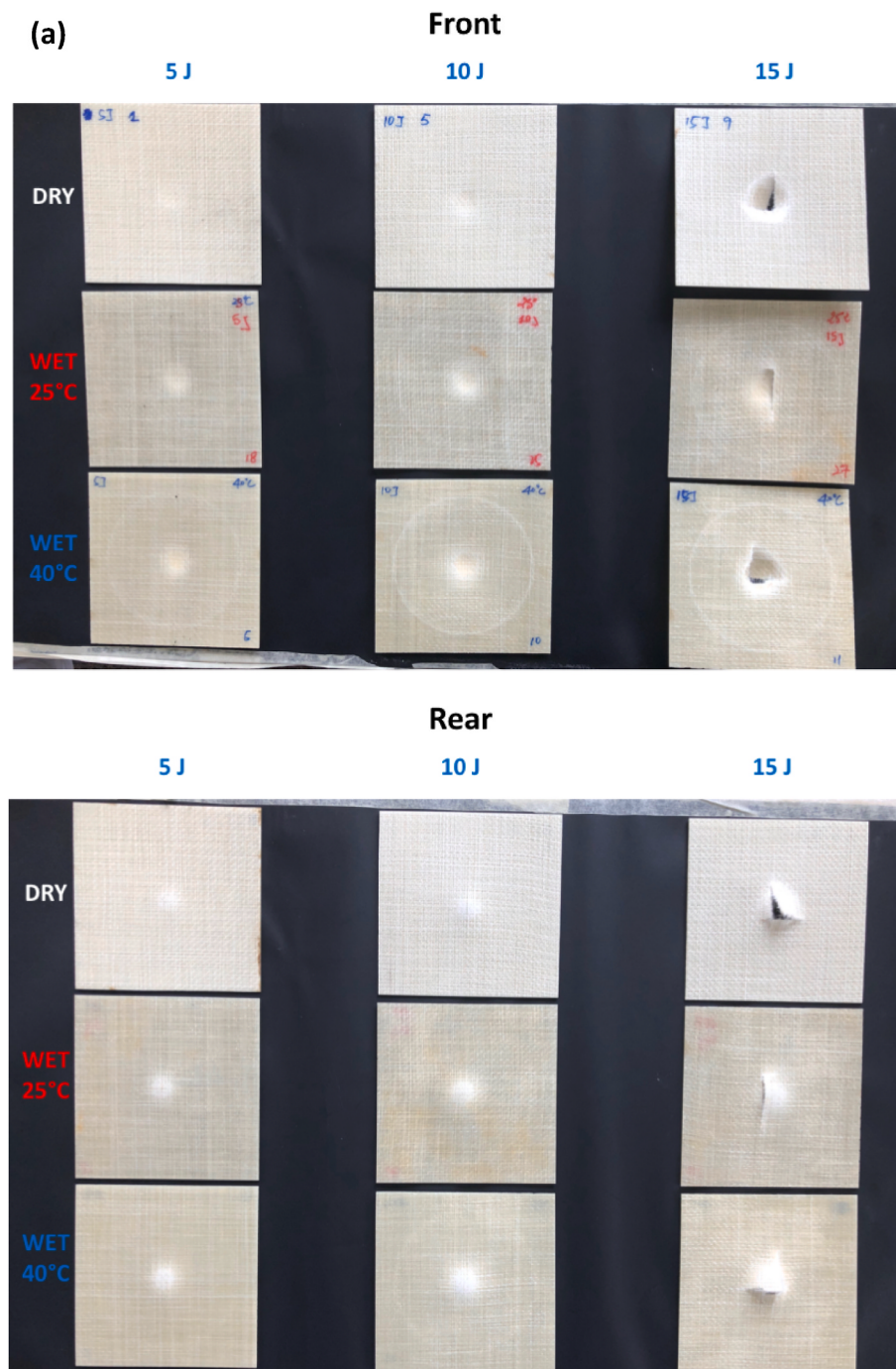
Fig. 9. Visual observations of the samples depicting their (a) front and (b) rear impacted faces respectively, with different energies (5 J, 10 J, 15 J) in dry, 25 °C and 40 °C wet aged conditions.
