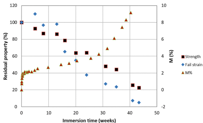
Fig. 14. Correlation between normalised loss in failure properties, after different immersion times at 40 °C, compared to initial unaged values and weight change.
