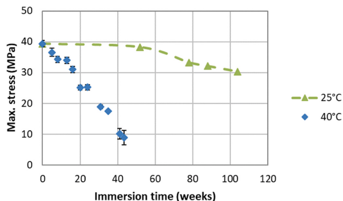
Fig. 15. Comparison between tensile response of unaged samples and samples after 12, 18, 21 and 24 months' 25 °C and 40 °C seawater immersion.
