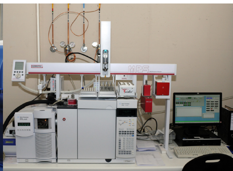
Chemical analyses on release of VOC, chemical composition and presence of hazardous components
